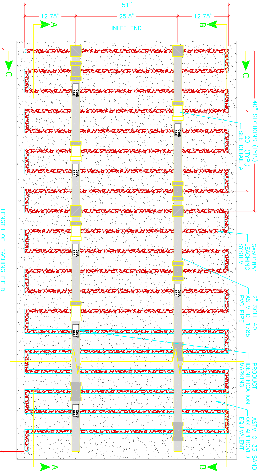
Geou1851 Leaching Trench - Plan View
